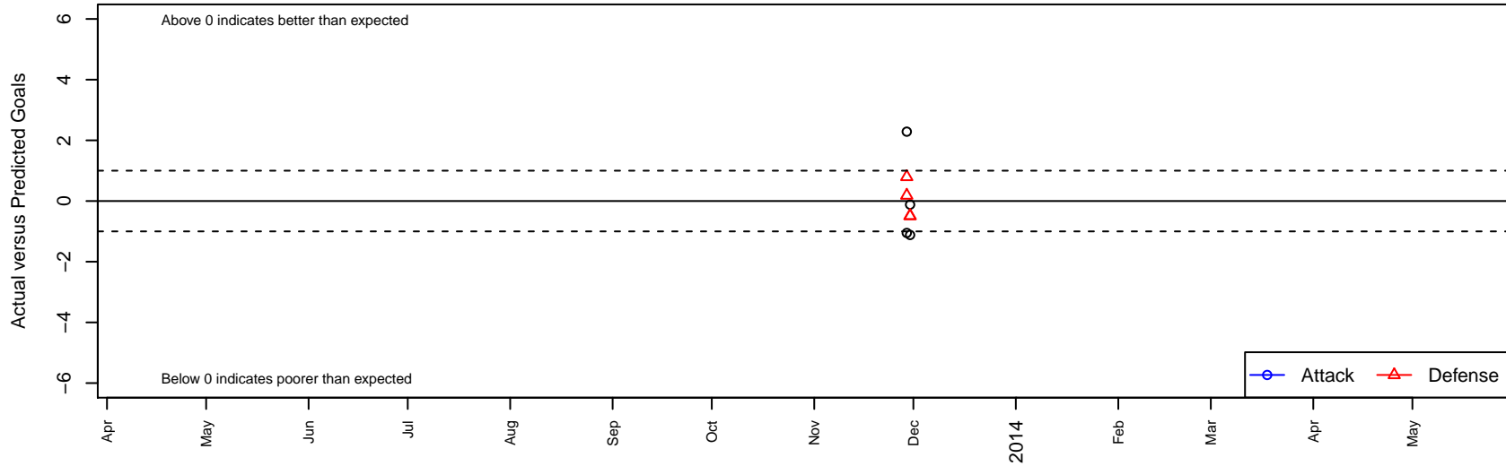
Marin FC 99 –Unk B98 Dots are actual minus expected GF (blue circles) and GA (red triangles). Blue line is smoothed change in attack strength. Red is smoothed change in defense strength.
